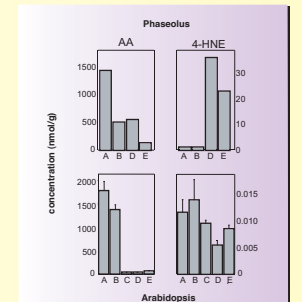
Figure 6. Variation in relative levels of AA and 4-HNE in tissue from leaves of P. vulgaris and A. thaliana inoculated with B. cinerea compared to control samples. A: non-inoculated plants under optimum growth conditions; B: non-inoculated plants under inoculation conditions; C: green areas of infected leaves ( Arabidopsis ); D: tissue adjacent to soft rot (chlorotic in Arabidopsis ); E, rotted tissue.
