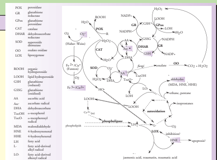
Figure 7. Simplified diagram illustrating oxidative reactions associated with the infection process.
